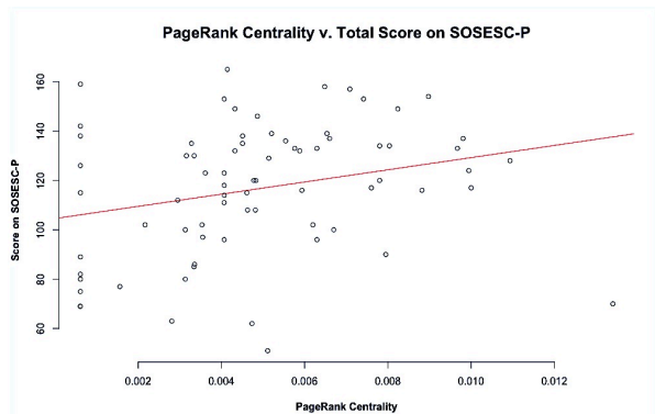
FIGURE 3. Scatterplot showing a linear correlation between PageRank centrality and total score on the SOSESC-P.
