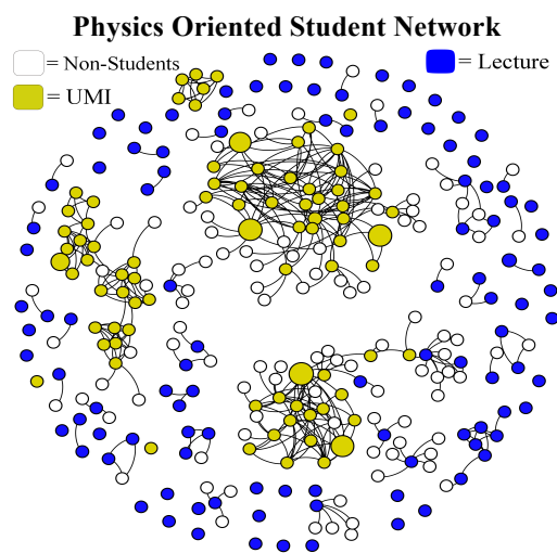
FIGURE 1. Sociogram showing students in the network. Labeled nodes specify the course type of those whose data was included in the study.
