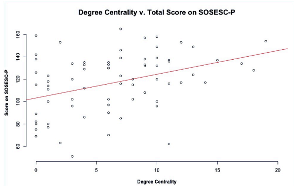
FIGURE 2. Scatterplot showing a linear correlation between degree centrality and total score on the SOSESC-P.
