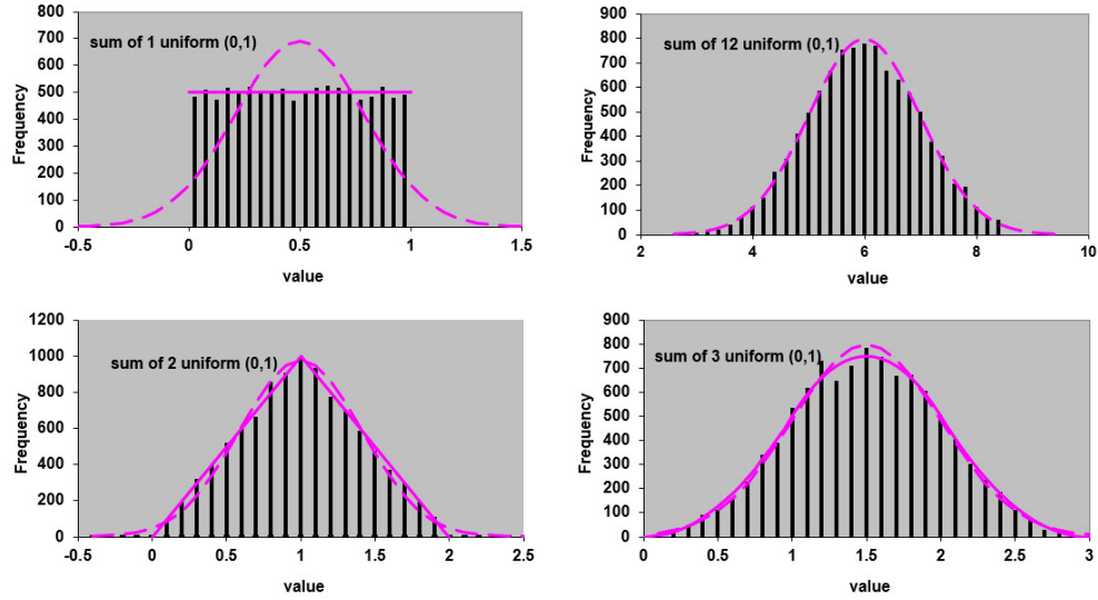
Figure 8.1: Counterclockwise from top left: Sample frequency distributions for 10,000 samples of the sum of 1, 2, 3 and 12 uniformly-distributed random numbers. The solid lines in the first three histograms are based on the true pdfs. The dotted lines in all four histograms are based on Gaussian pdfs with that histogram's true mean and variance.
