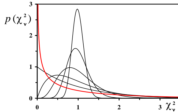
Figure 9.2: The reduced chi-square pdfs p(\chi^2_\nu) for degrees of freedom (dof) 1, 2, 4, 10, 30, 100. The tall distribution peaking at \chi^2_\nu = 1 is for dof = 100. The curves get broader and lower as the dof decrease. For dof = 1, the distribution (red) is singular at zero.
